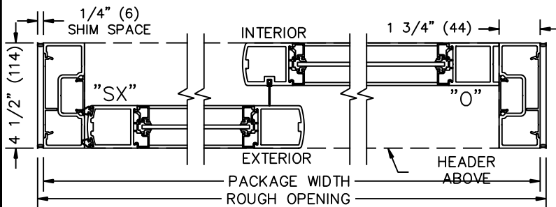
② HORIZONTAL SECTION
