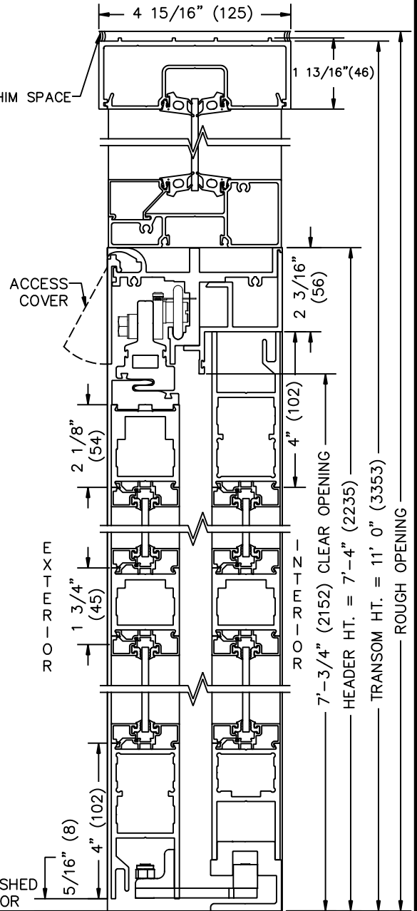
① VERTICAL SECTION
