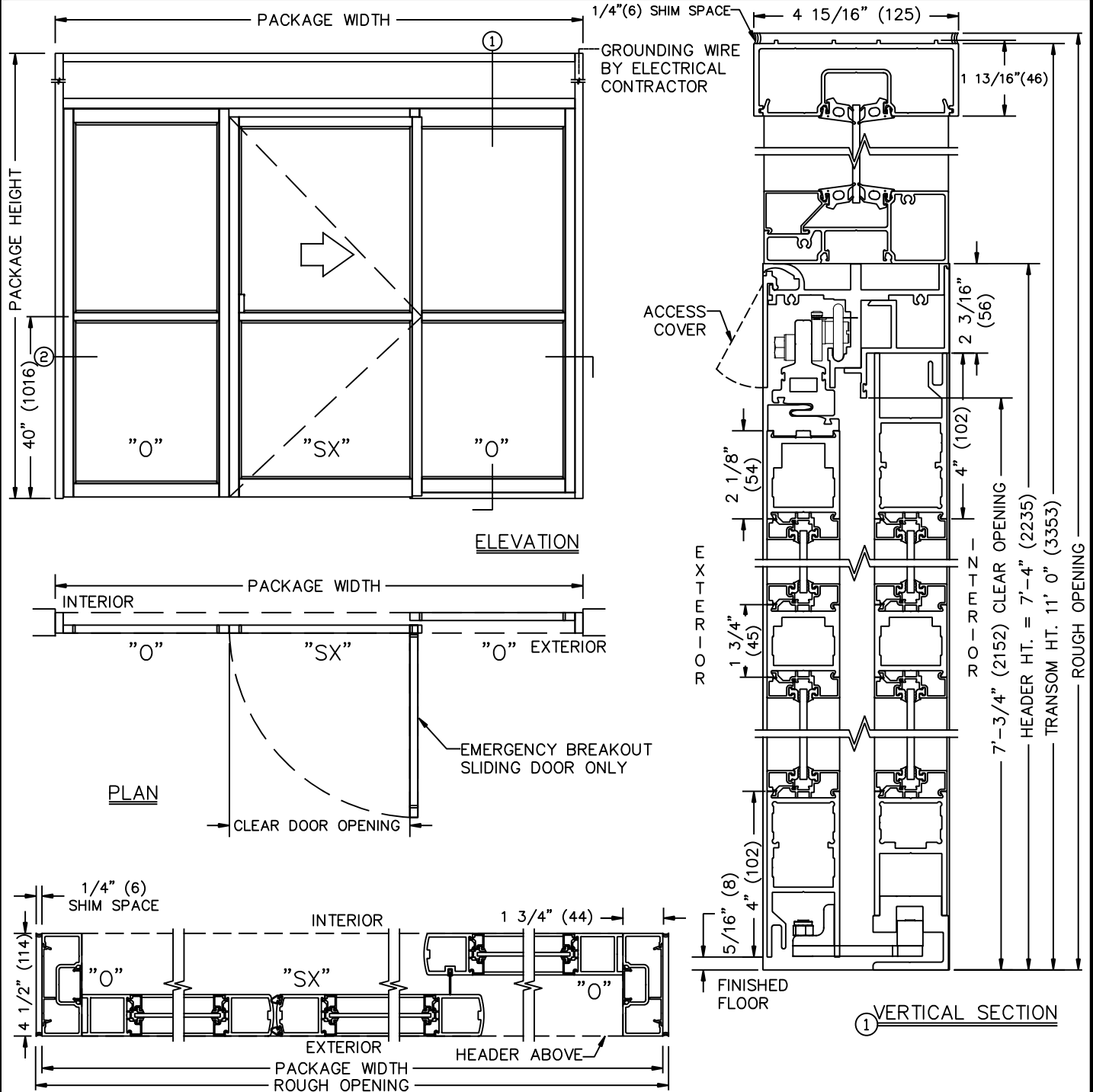
② HORIZONTAL SECTION
