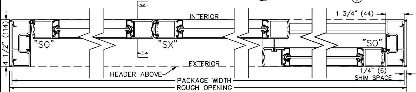
② HORIZONTAL SECTION
