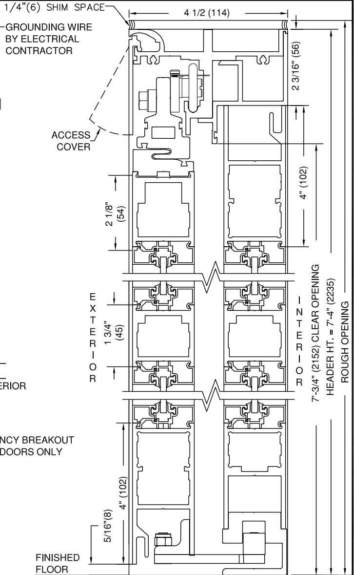
① VERTICAL SECTION
