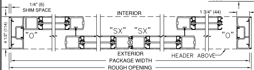
② HORIZONTAL SECTION
