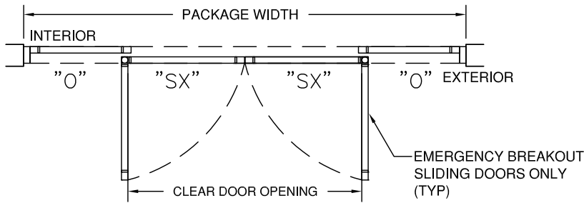
PLAN
