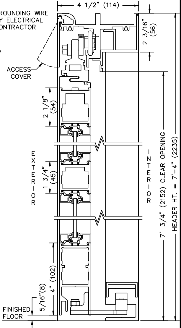
① VERTICAL SECTION
