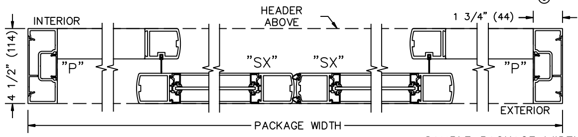
② HORIZONTAL SECTION
