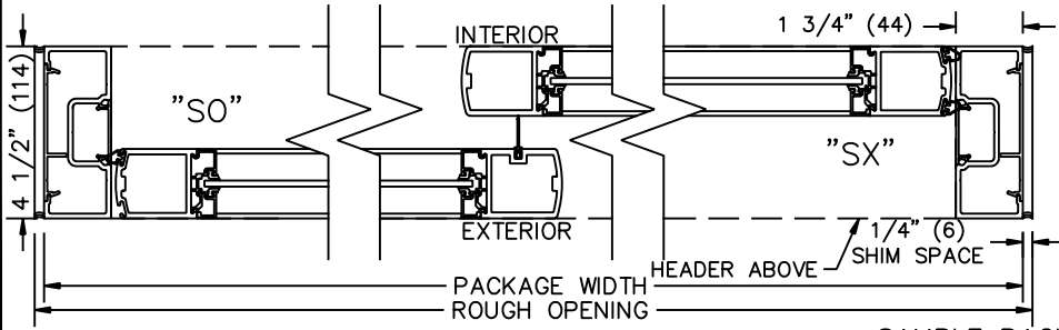
2 HORIZONTAL SECTION
