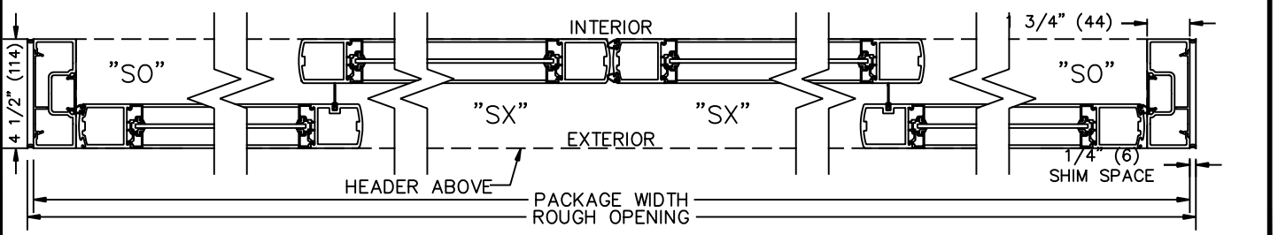
② HORIZONTAL SECTION
