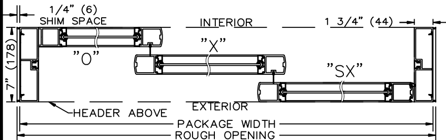
2 HORIZONTAL SECTION
