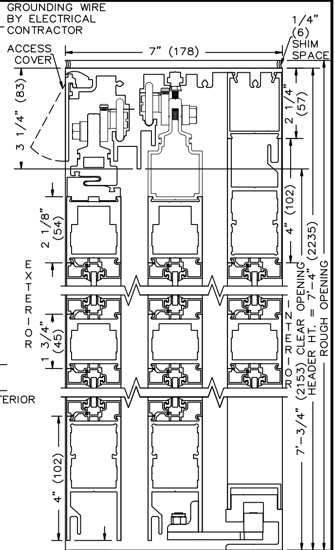
1 VERTICAL SECTION
