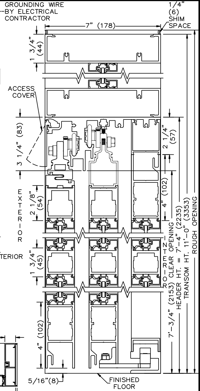
VERTICAL SECTION
