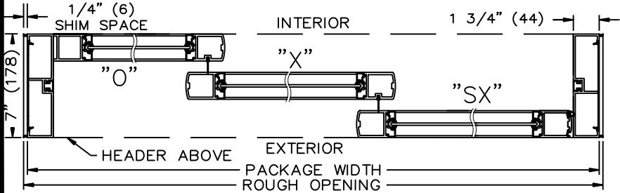
HORIZONTAL SECTION
