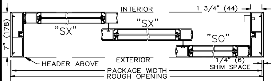
HORIZONTAL SECTION
