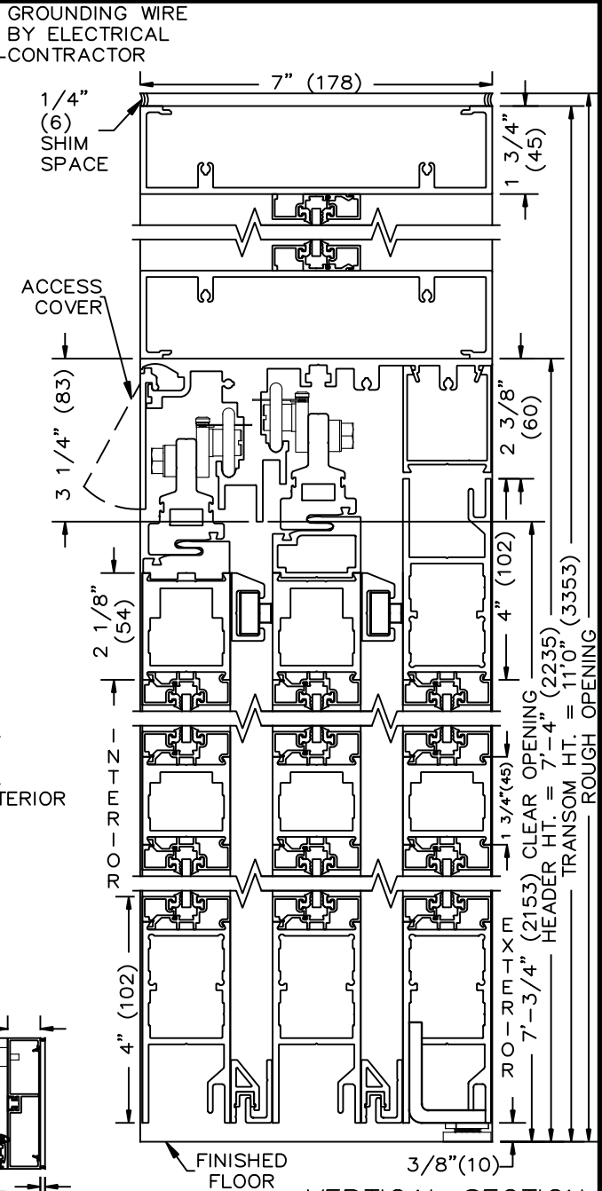
VERTICAL SECTION
